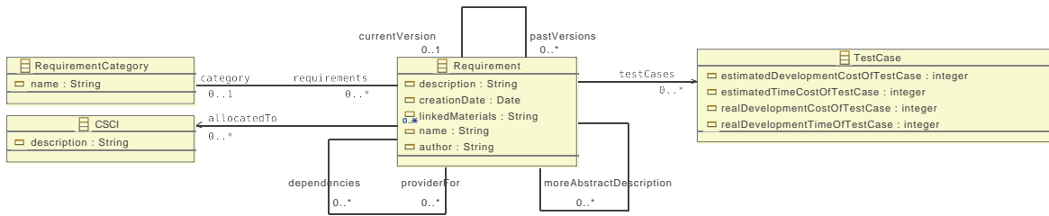
Figure 4: The requirement concept
