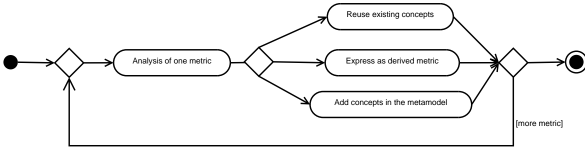
Figure 2: Our metric-driven metamodeling process
